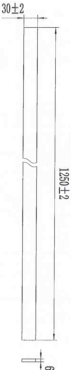
BACK RING WELDING DETAIL 衬圈焊接详图 NO SCALE
